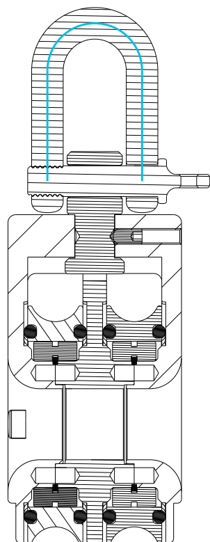
SECTION XSEC0001-XSEC0001 SCALE 3:4
